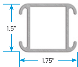
Standard extrusion for smaller sizes.
